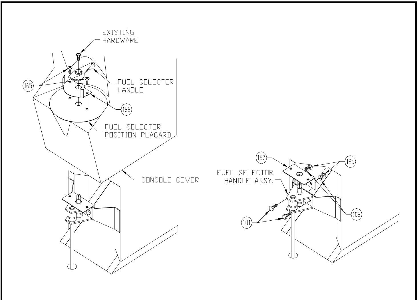
Figure 1 - Fuel Selector Stop Installation Detail
